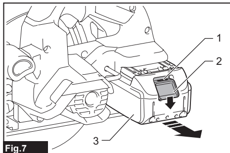
Fig. 7 1. Red indicator 2. Button 3. Battery cartridge
